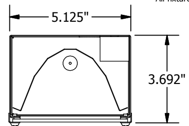
5.125" 3.692" END VIEW
