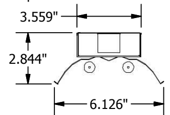
2-Lamp T5HO Strip inside Enclosure
