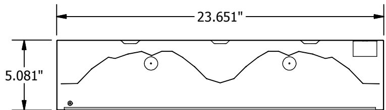
LS-HCB (2 Lamp T8)
