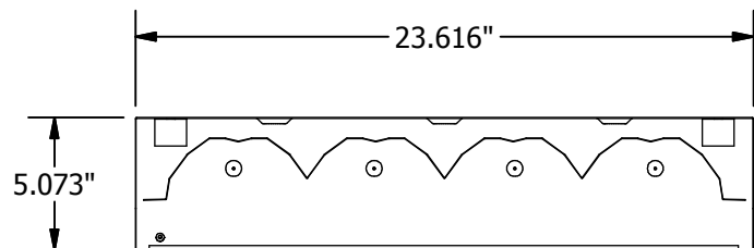
END VIEW
