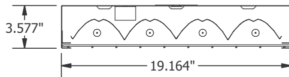
END VIEW
